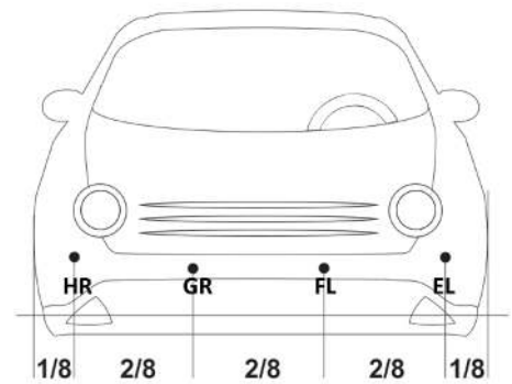
For Front: 4 sensors installation
