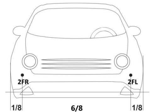
For Front: 2 sensors installation
