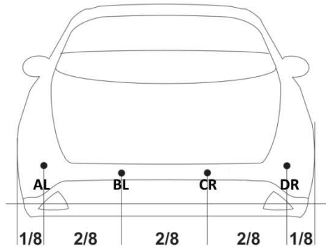
For Rear: 4 sensors installation
