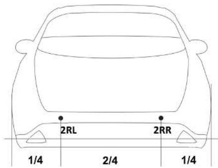
For Rear: 2 sensors installation
